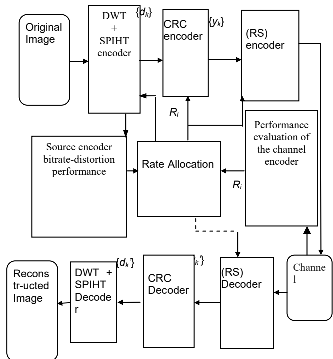
Fig.8. Applied to the image transmission system
