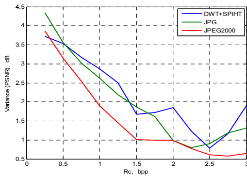
Fig.7. PSNR variation of the 15 selected natural test images
