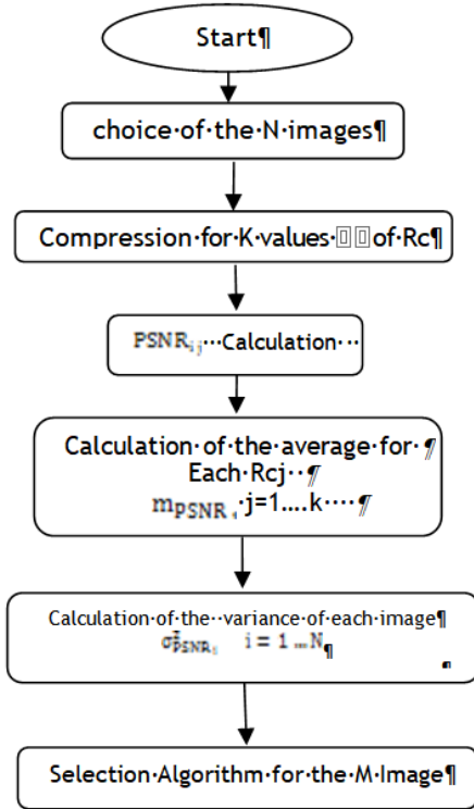
Fig.6. Chart of Selection Algorithm for Test Images
