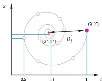
Fig.3. Spiral updating position
