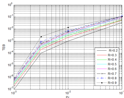
Fig. 4.error Bit rate in function of error probability.
