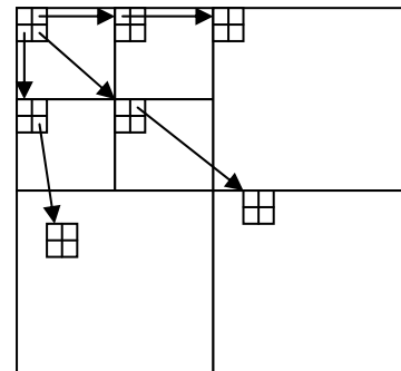
Fig.2. Tree structure of wavelet coefficients in the case of SPIHT
