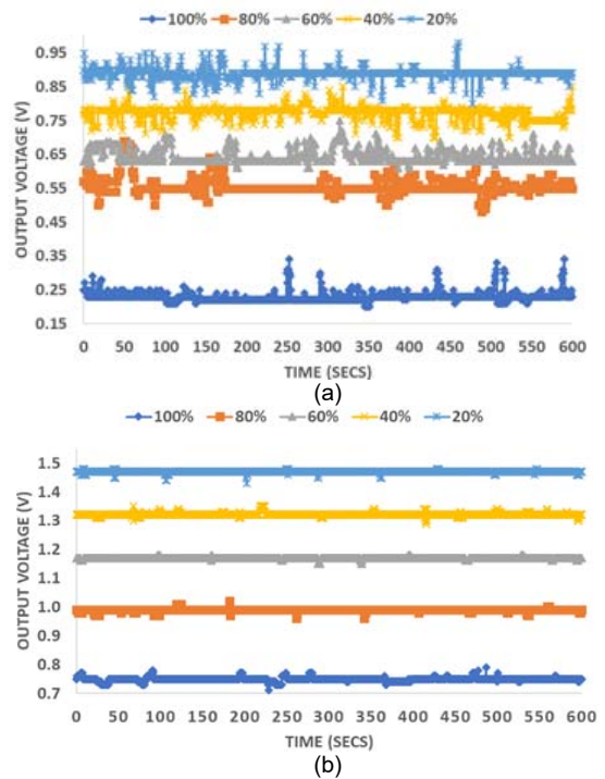
Fig.6. Stability graph for; a) Uncoated glass and b) HEC/PVDF coated glass
