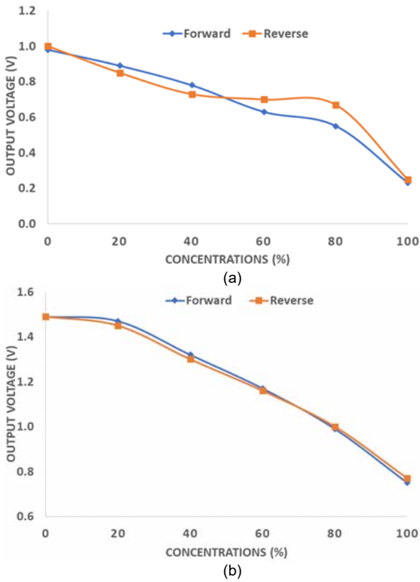
Fig.4. Hysteresis graph for; a) Uncoated glass and b) HEC/PVDF coated glass
