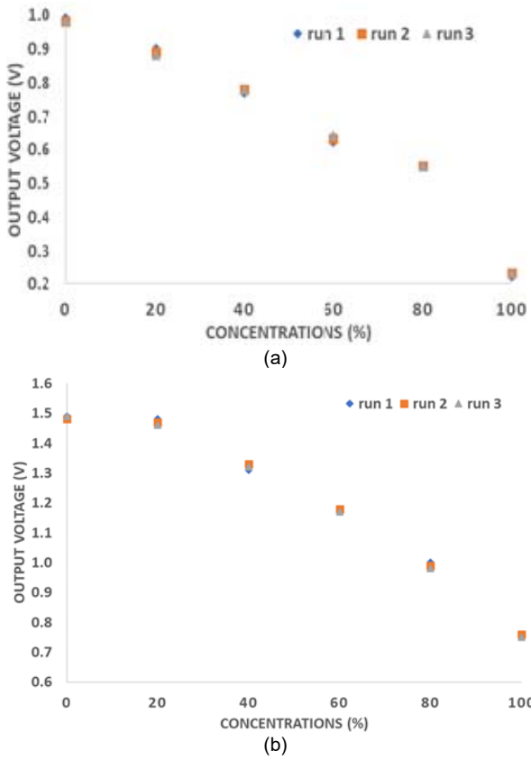
Fig.3. Reproducibility of; a) Uncoated glass and b) HEC/PVDF coated glass
