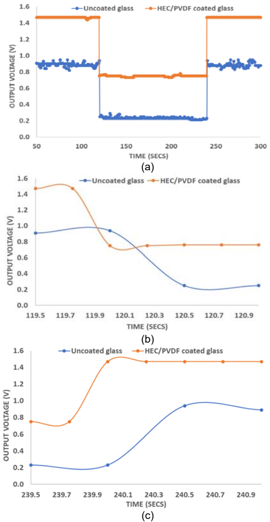
Fig.5. Time reponse for; a) Overall, b) Response time and c) Recovery time
