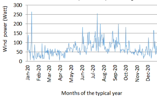
Fig.9. Wind electrical power output at Maginti
