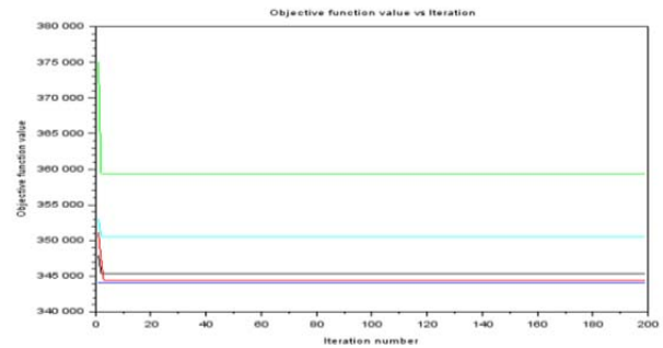
Fig.10. Convergence process with BSG Starcraft PSO
