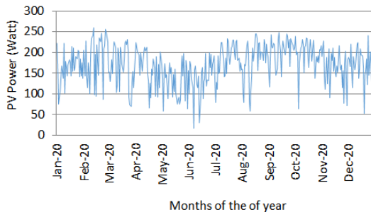
Fig. 8. Solar-irradiation electrical power output at Maginti
