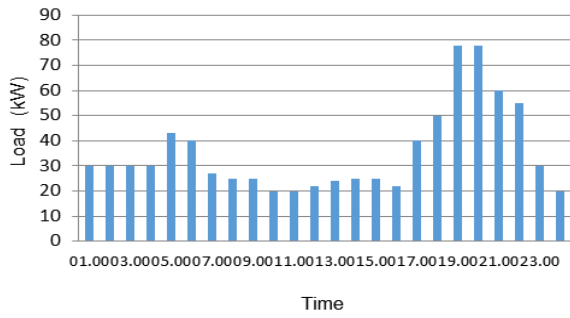
Fig. 5. Load profile in Maginti
