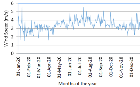
Fig.4. Variation wind speed in Maginti
